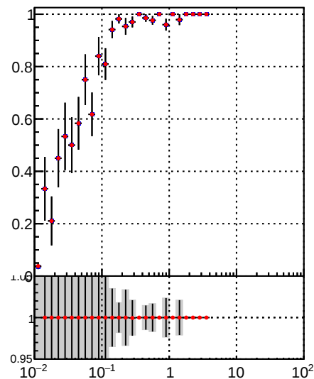
—•— /data2/legianni/BDT-vs-DNN/real-BDT/CMSSW_13_0_0_pre4/src/DQM_mkFit_time —•— DQM_TT_mkFit-DQM_time_mod
