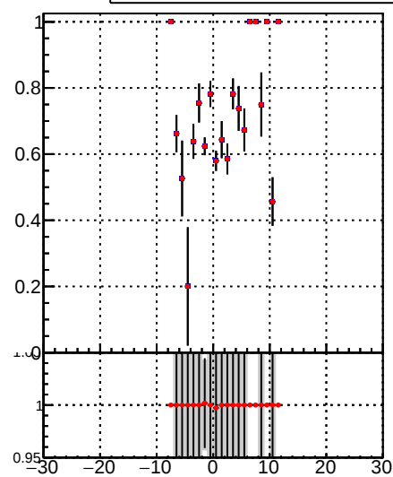
—•— /data2/legianni/BDT-vs-DNN/real-BDT/CMSSW_13_0_0_pre4/src/DQM_mkFit_time —•— DQM_TT_mkFit-DQM_time_mod
