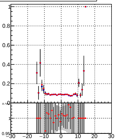
/data2/legianni/BDT-vs-DNN/real-BDT/CMSSW_13_0_0_pre4/src/DQM_mkFit_time
