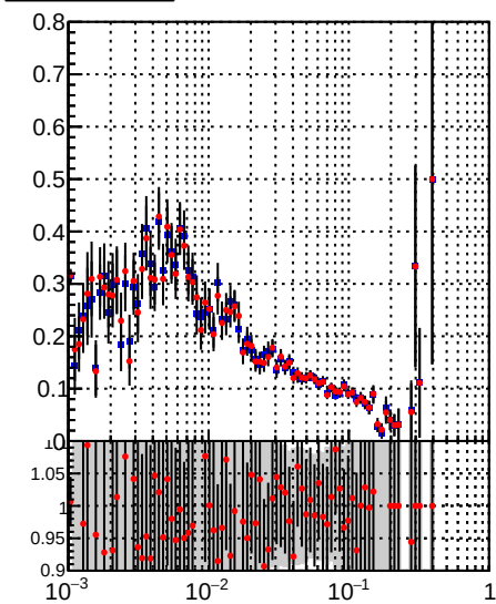
/data2/legianni/BDT-vs-DNN/real-BDT/CMSSW_13_0_0_pre4/src/DQM_mkFit_time DQM_TT_mkFit-DQM_time_mod
