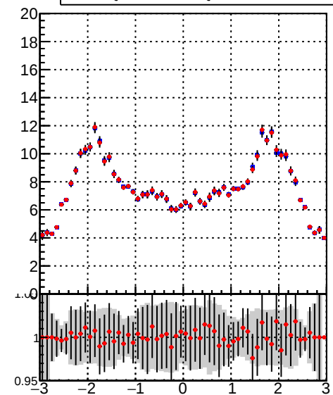
/data2/legianni/BDT-vs-DNN/real-BDT/CMSSW_13_0_0_pre4/src/DQM_mkFit_time DQM_TT_mkFit-DQM_time_mod mean hit
