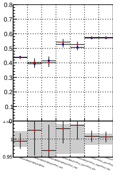
Fake rate vs. —•— /data2/legianni/BDT-vs-DNN/real-BDT/CMSSW_13_0_0_pre4/src/DQM_mkFit_time —•— DQM_TT_mkFit-DQM_time_mod
