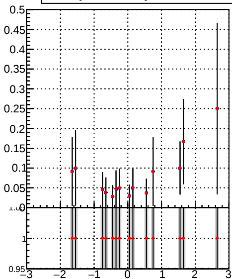
—•— /data2/legianni/BDT-vs-DNN/real-BDT/CMSSW_13_0_0_pre4/src/DQM_mkFit_time —•— DQM_TT_mkFit-DQM_time_mod
