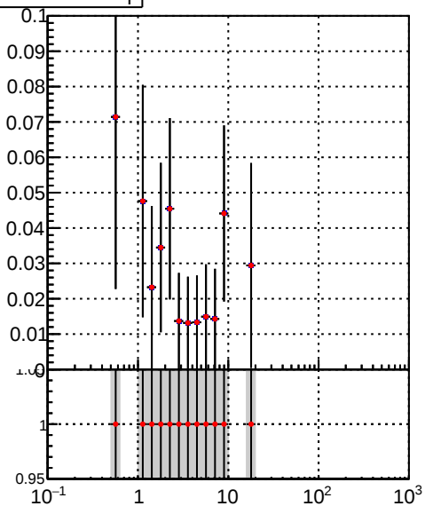
—•— /data2/legianni/BDT-vs-DNN/real-BDT/CMSSW_13_0_0_pre4/src/DQM_mkFit_time —•— DQM_TT_mkFit-DQM_time_mod
