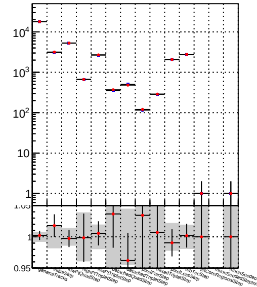
Number —●— DQM_TT__mkFit-DQM_time_mod
