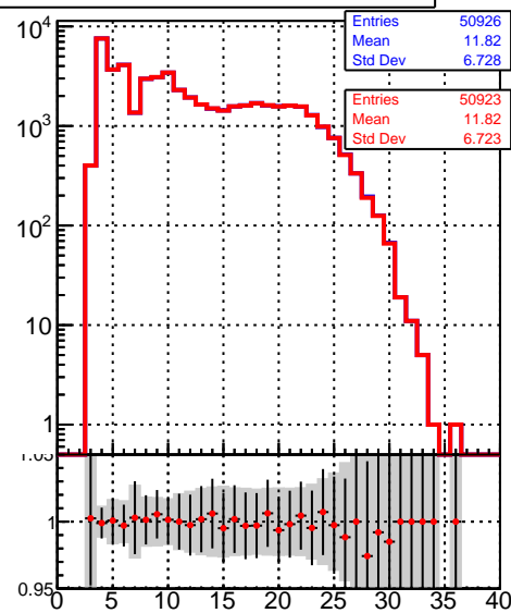
Legend /data2/legianni/BDT-vs-DNN/real-BDT/CMSSW_13_0_0_pre4/src/DQM_mkFit_time
