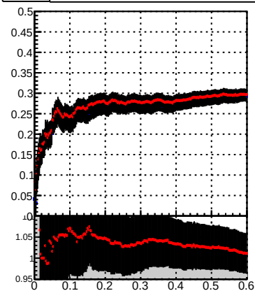
Fake rate — DQM_TT__mkFit-DQM_time_mod
