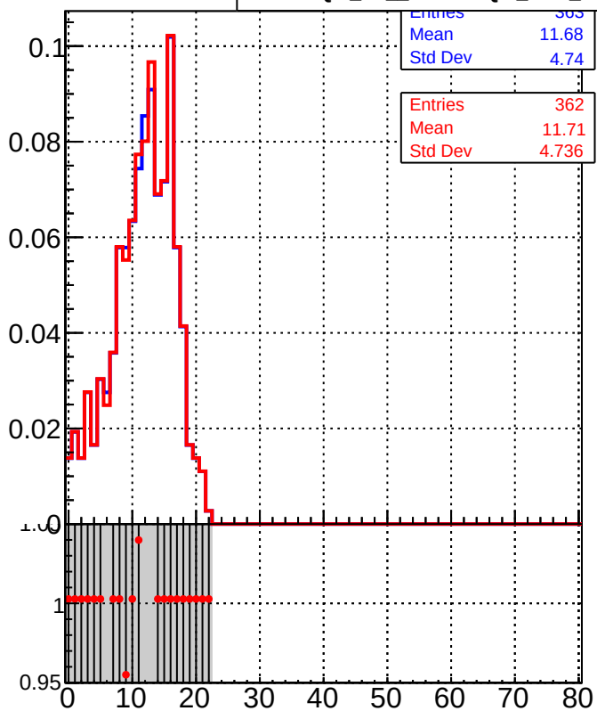
/data2/legianni/BDT-vs-DNN/real-BDT/CMSSW_13_0_0_pre4/src/DQM_mkFit_time DQM_TT_mkFit-DQM_time_mod
