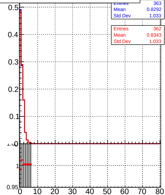
/data2/legianni/BDT-vs-DNN/real-BDT/CMSSW_13_0_0_pre4/src/DQM_mkFit_time DQM_TT_mkFit-DQM_time_mod
