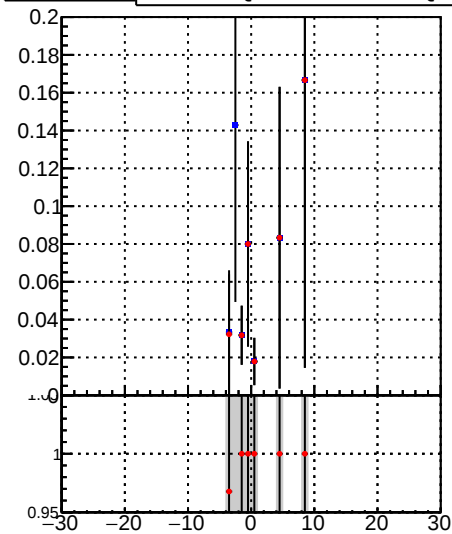
Fake rate vs v DQM_TT_mkFit-DQM_time_mod /data2/legianni/BDT-vs-DNN/real-BDT/CMSSW_13_0_0_pre4/src/DQM_mkFit_time DQM_TT_mkFit-DQM_time_mod
