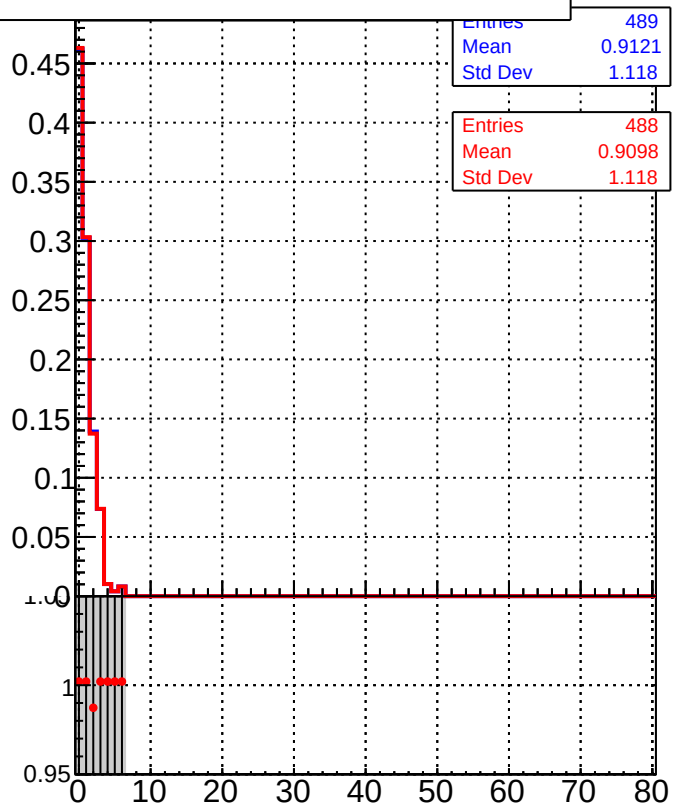
/data2/legianni/BDT-vs-DNN/real-BDT/CMSSW_13_0_0_pre4/src/DQM_mkFit_time DQM_TT_mkFit-DQM_time_mod
