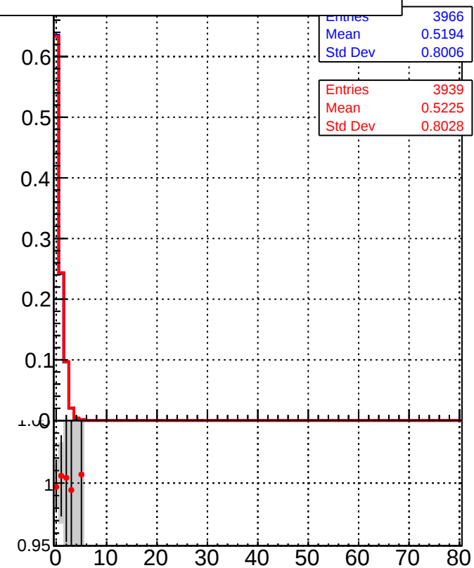
/data2/legianni/BDT-vs-DNN/real-BDT/CMSSW_13_0_0_pre4/src/DQM_mkFit_time DQM_TT_mkFit-DQM_time_mod
