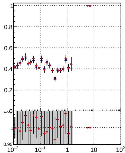
—•— /data2/legianni/BDT-vs-DNN/real-BDT/CMSSW_13_0_0_pre4/src/DQM_mkFit_time —•— DQM_TT_mkFit-DQM_time_mod
