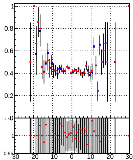
—•— /data2/legianni/BDT-vs-DNN/real-BDT/CMSSW_13_0_0_pre4/src/DQM_mkFit_time —•— DQM_TT_mkFit-DQM_time_mod
