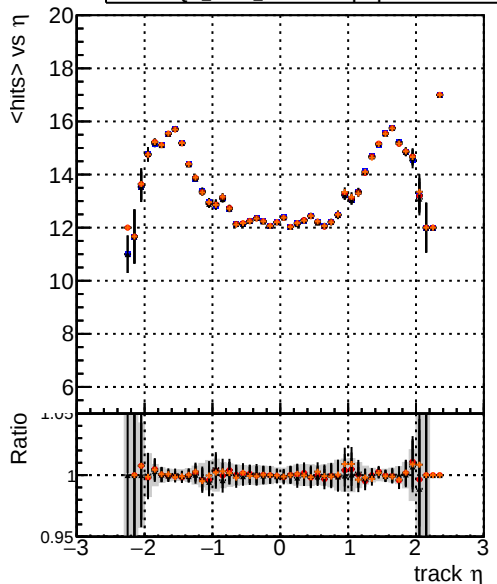
mean hit Legend: - DQM_mkFit_TToriginal (blue line) - DQM_mkFit_TTNEW50 (red line with dots) - DQM_mkFit_TTNEW50-chi2 (black line with dots) - DQM_mkFit_TTNEW50-dpdg (orange line with dots)
