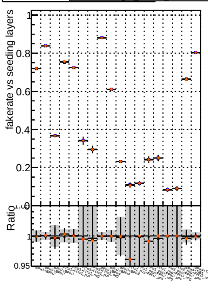
Fake rate vs. Legend: DSM mkFit TToriginal DSM mkFit TTNEW50 DSM mkFit TTNEW50-8b12
