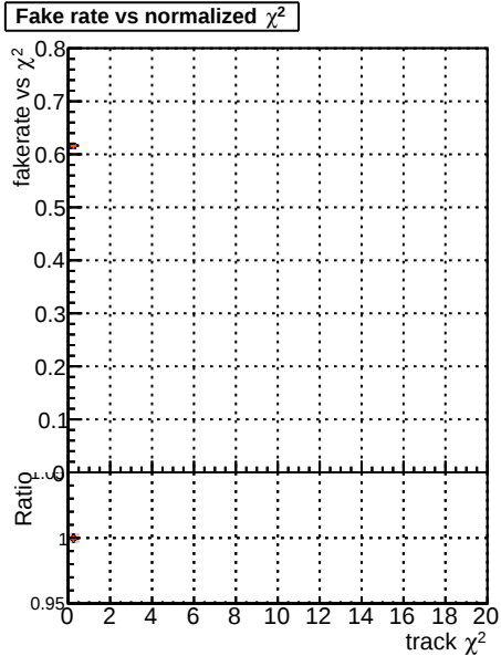
Fake rate vs. Legend: DSM mkFit TToriginal DSM mkFit TTNEW50 DSM mkFit TTNEW50-8b12
