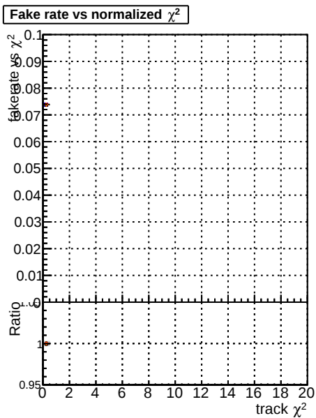
Fake rate vs. \chi^2 Legend: DSM mkFit TToriginal DSM mkFit TTnew50 DSM mkFit TTnew50-8b12
