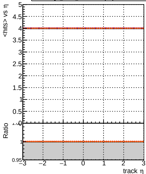
mean hits DQM_mkFit_TToriginal DQM_mkFit_TTNEW50 DQM_mkFit_TTNEW50-chi2 DQM_mkFit_TTNEW50-dpdq
