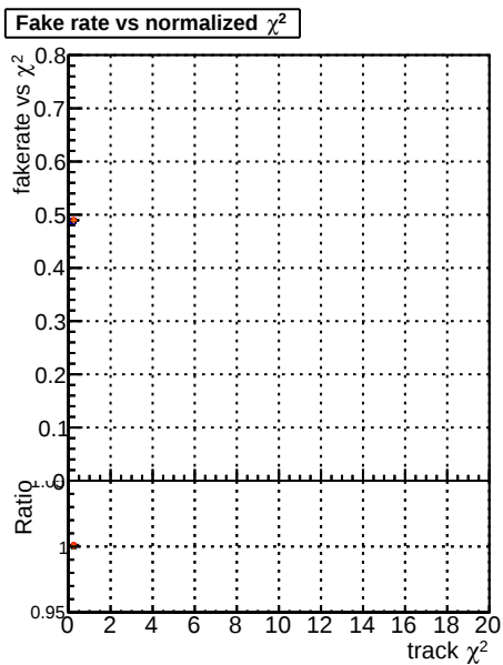
Fake rate vs. Legend Series Blue line with dots BGM mkt fit T original Red line with dots BGM mkt fit T NEW50-sh12 Orange line with dots BGM mkt fit T NEW50-sh12
