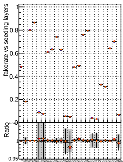
Fake rate vs. Legend Series Blue line with dots BGM mkt fit T original Red line with dots BGM mkt fit T NEW50-sh12 Orange line with dots BGM mkt fit T NEW50-sh12
