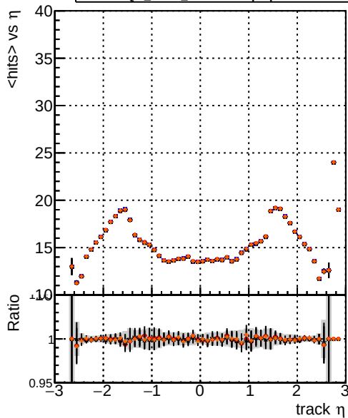
Legend: DOM_mkFit_TToriginal DOM_mkFit_TTNEW50 DOM_mkFit_TTNEW50-chi2 DOM_mkFit_TTNEW50-dpdq mean hit
