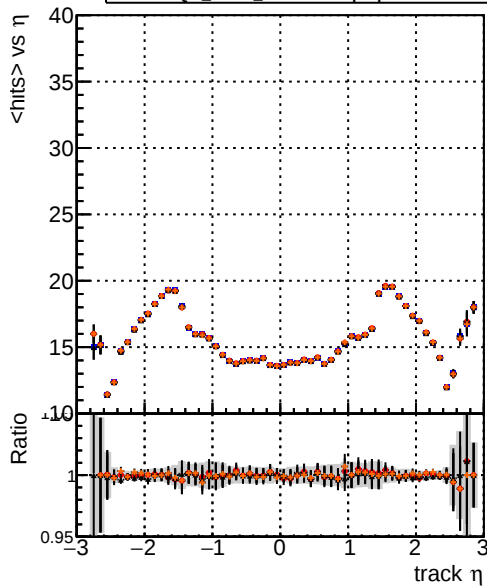
mean hit Legend: DQM_mkFit_TToriginal (blue), DQM_mkFit_TTNEW50 (red), DQM_mkFit_TTNEW50-chi2 (black), DQM_mkFit_TTNEW50-dpdq (orange)
