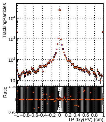
N of sim DQM_mkFit_TToriginal DQM_mkFit_TTNEW50 DQM_mkFit_TTNEW50-chi2 DQM_mkFit_TTNEW50-dpdq
