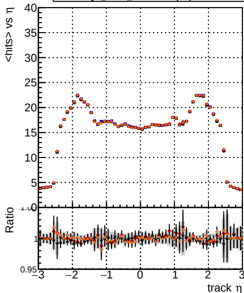
mean hit — DQM_mkFit_TToriginal — DQM_mkFit_TTNEW50 — DQM_mkFit_TTNEW50-chi2 — DQM_mkFit_TTNEW50-dp2q
