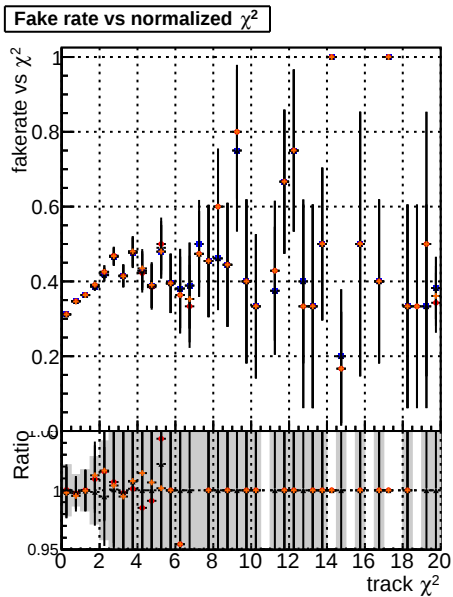
Fake rate vs. \chi^2 Legend: BQM, mkFit, T, Toriginal, TNEW50
