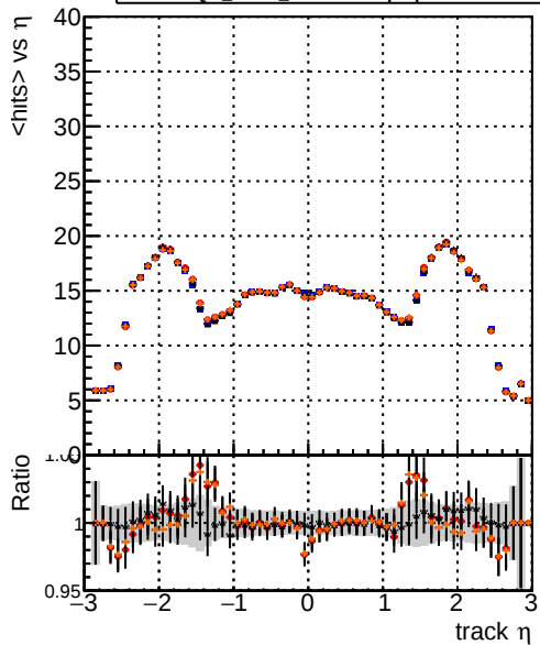
mean hit Legend: DQM_mkFit_TToriginal (blue line), DQM_mkFit_TTNEW50 (red line), DQM_mkFit_TTNEW50-chi2 (black line), DQM_mkFit_TTNEW50-dp2q (orange line)
