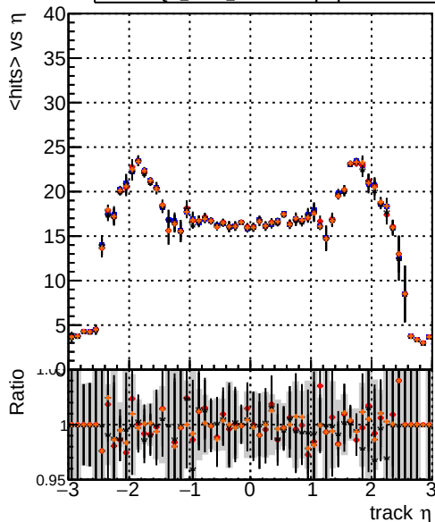
Legend: DQM_mkFit_TToriginal (blue line with dots), DQM_mkFit_TTNEW50 (red line with dots), DQM_mkFit_TTNEW50-chi2 (black line with dots), DQM_mkFit_TTNEW50-dp2q (orange line with dots) mean hit
