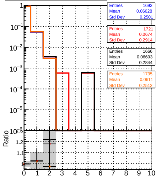
Legend: DQM_mkFit_TToriginal (blue line with dots), DQM_mkFit_TTNEW50 (red line with dots), DQM_mkFit_TTNEW50-chi2 (black line with dots), DQM_mkFit_TTNEW50-dp2q (orange line with dots) mean hit
