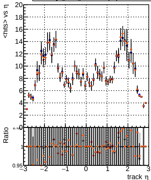
mean hit DQM_mkFit_TToriginal DQM_mkFit_TTNEW50 DQM_mkFit_TTNEW50-chi2 DQM_mkFit_TTNEW50-dpdaq
