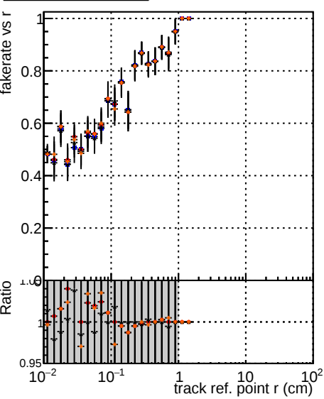
Fake rate vs v Legend: DOM mktFit Toriginal DOM mktFit NEW50-chi2 DOM mktFit NEW50-apdq
