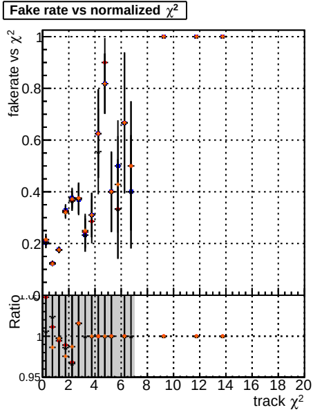
Fake rate vs. BQM mklfit Toriginal BQM mklfit TNEW50 BQM mklfit TNEW50-8b12
