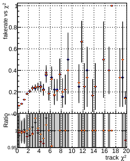
Fake rate vs. \chi^2 for different track selection criteria
