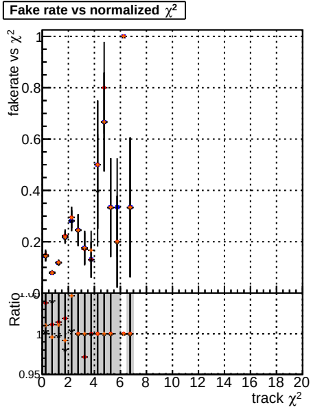
Fake rate vs. BQM mkFit TTest TTest50 NEW50-shi2
