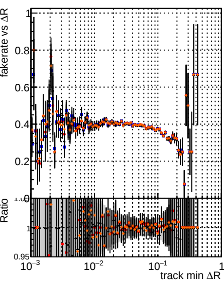
Fake rate vs \Delta R(\text{track, jet}) DOM mktFit Original DOM mktFit NEW50 chi2 DOM mktFit NEW50-apdq
