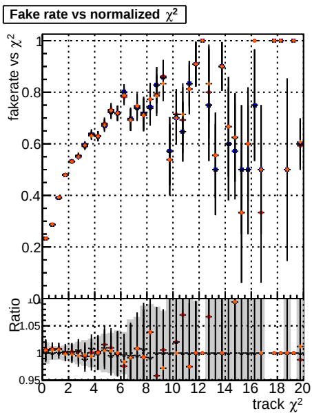
Fake rate vs. \chi^2 Legend: BQM mkFit TTT original
