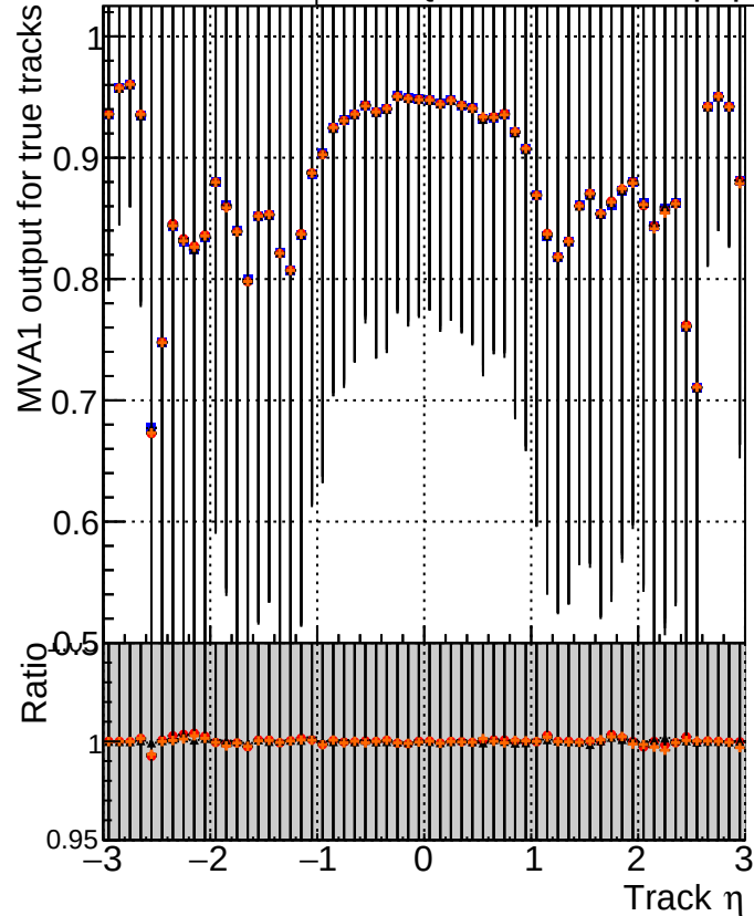
MVA1 of associated tracks (recoToSim) vs. track \eta Legend: DQM_mkFit_TToriginal (blue square) DQM_mkFit_TTNEW50 (red diamond) DQM_mkFit_TTNEW50-chi2 (black triangle) DQM_mkFit_TTNEW50-dpdq (orange diamond)
