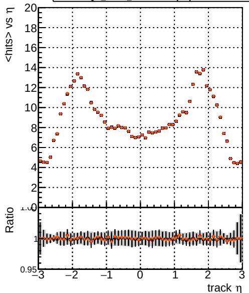
mean hit DQM_mkFit_TToriginal DQM_mkFit_TTNEW50 DQM_mkFit_TTNEW50-chi2 DQM_mkFit_TTNEW50-dp2q
