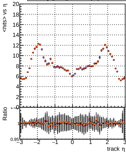
DQM_mkFit_TToriginal DQM_mkFit_TTNEW50 DQM_mkFit_TTNEW50-chi2 DQM_mkFit_TTNEW50-dpdaq mean hit
