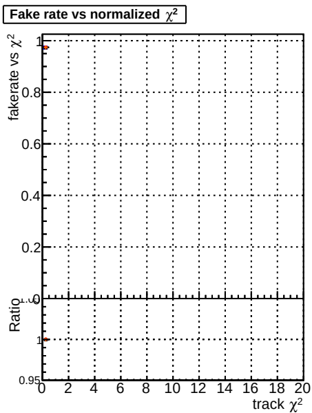
Fake rate vs. \chi^2 Legend: BBM mkFit TToriginal BBM mkFit TTNEWS BBM mkFit TTNEWS_dnd
