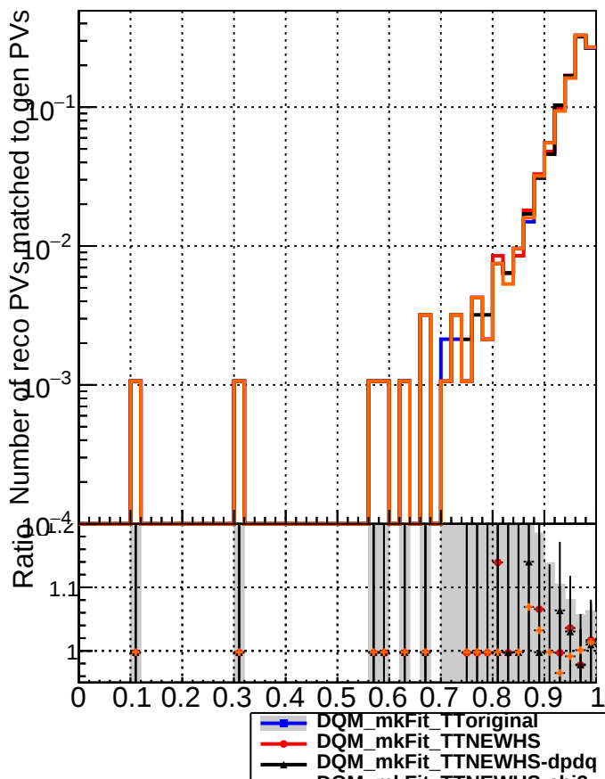
RecoPVAssoc2GenPVmatched_missing
