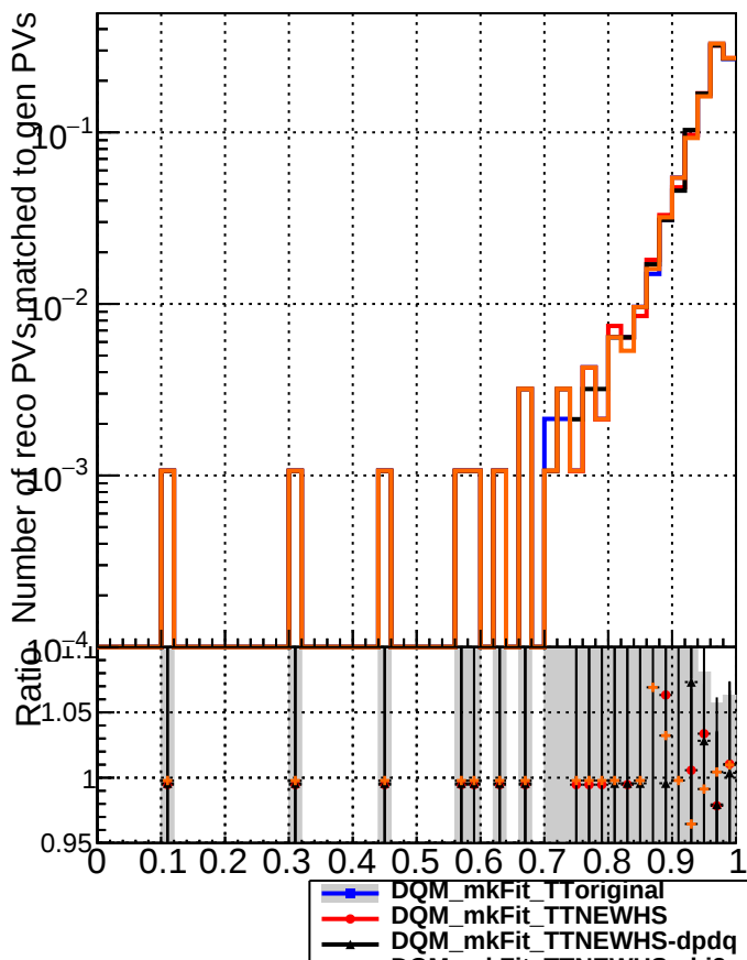
RecoPVAssoc2GenPVmatched_missing
