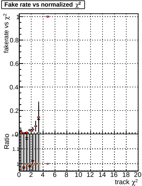
Fake rate vs. Legend: BBM mkFit TToriginal BBM mkFit TTNEWS BBM mkFit TTNEWS dnd
