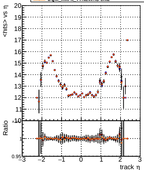
mean hit Legend: DQM_mkFit_TToriginal (blue line) DQM_mkFit_TTNEUHS (red line) DQM_mkFit_TTNEUHS-dpdq (black line) DQM_mkFit_TTNEUHS-chi2 (orange line)
