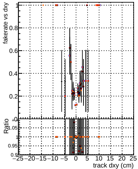
—•— BSM mktFit TToriginal —•— BSM mktFit TTNEWS dnd1 —•— BSM mktFit TTNEWS dnd2
