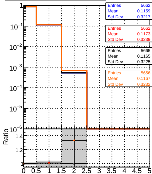
mean hit DQM_mkFit_TToriginal DQM_mkFit_TTNEWHS DQM_mkFit_TTNEWHS-dpdq DQM_mkFit_TTNEWHS-chi2
