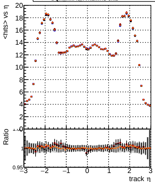
Legend: DQM_mkFit_TToriginal (blue), DQM_mkFit_TTNEUHS (red), DQM_mkFit_TTNEUHS-dpdq (black), DQM_mkFit_TTNEUHS-chi2 (orange) mean hit
