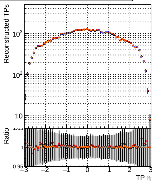
N of associated tracks (simToReco) vs eta
