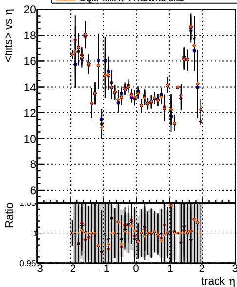
Legend: DOM_mkFit_TToriginal DOM_mkFit_TTNEWHs DOM_mkFit_TTNEWHs-dpdq DOM_mkFit_TTNEWHs-chi2
