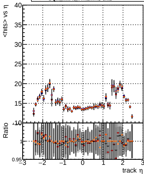
— DQM_mkFit_TToriginal — DQM_mkFit_TTNEWS — DQM_mkFit_TTNEWS-dpdq — DQM_mkFit_TTNEWS-chi2 mean hit
