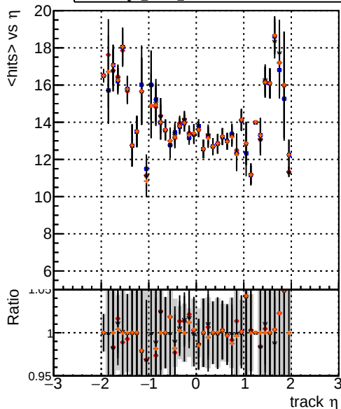
Legend: DOM_mkFit_TToriginal DOM_mkFit_TTNEUHS DOM_mkFit_TTNEUHS-dpdq DOM_mkFit_TTNEUHS-chi2 mean hit
