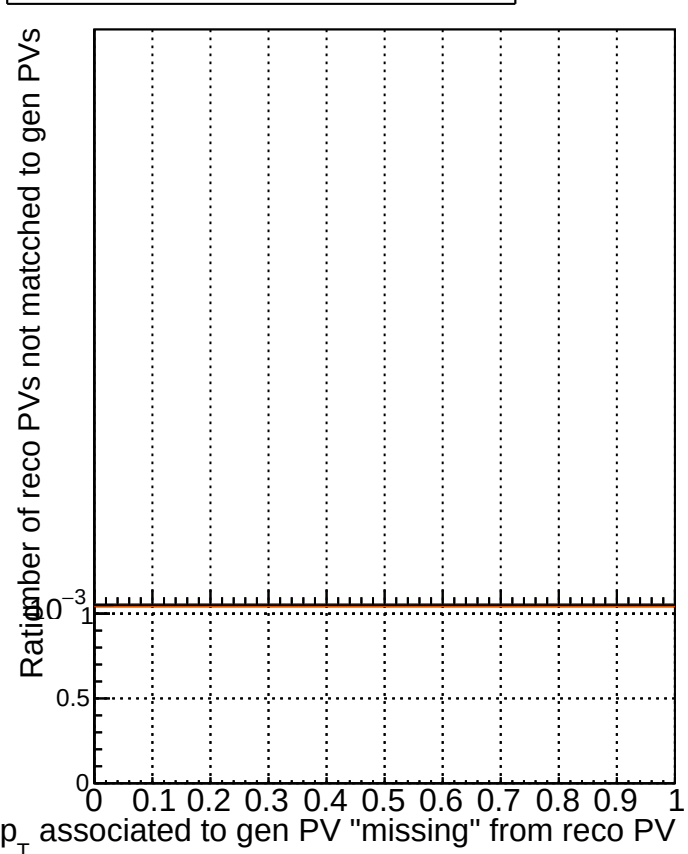
RecoPVAssoc2GenPVNotMatched_missing
