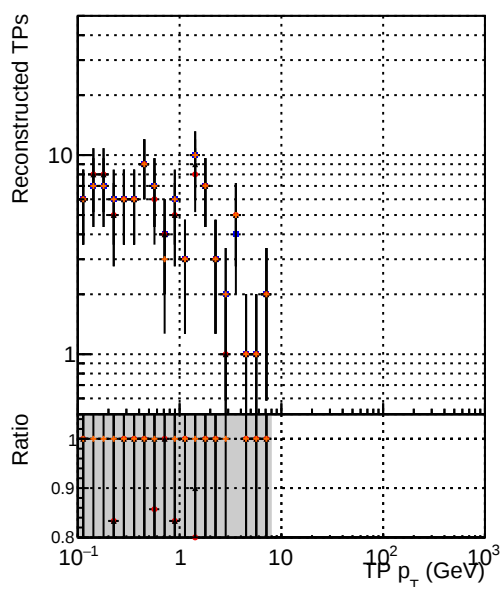
Legend: DQM_mkFit_TToriginal (blue circle), DQM_mkFit_TTNEUHS (red circle), DQM_mkFit_TTNEUHS-dpdq (black triangle), DQM_mkFit_TTNEUHS-chi2 (orange circle)
